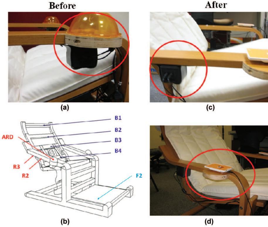
FIGURE 12. Photographs showing the modifications to the chair: (a) original version; (b) schematic drawing of the chair (F2 = footrest; B1-B4 = backrest; R2, R3 = armrest; ARD = plastic dome); (c) new location of the Nimzy speakers; (d) plastic dome was replaced by Xa-10 flat panel speakers from TDK. (Color figure available online.)
